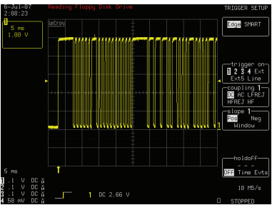
1 Remote control eye data FU3 Pin3
