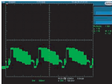
⑥ CVBS(Color-bar) Pin (MIC1-VC4, VIC1-VR22)
