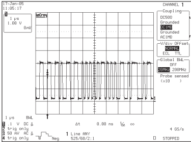
DIGITAL AUDIO DATA AIC1 (Pin2,4,6,13)
