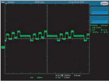
6 Pb(Color-bar) Pin-VR44
