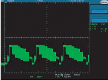
4 CVBS(Color-bar) Pin (MIC1-VC4,VIC1-VR22)
