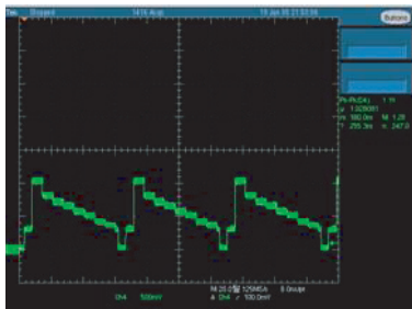
① Y(Color-bar) Pin (MIC1-VE26, VR37)
